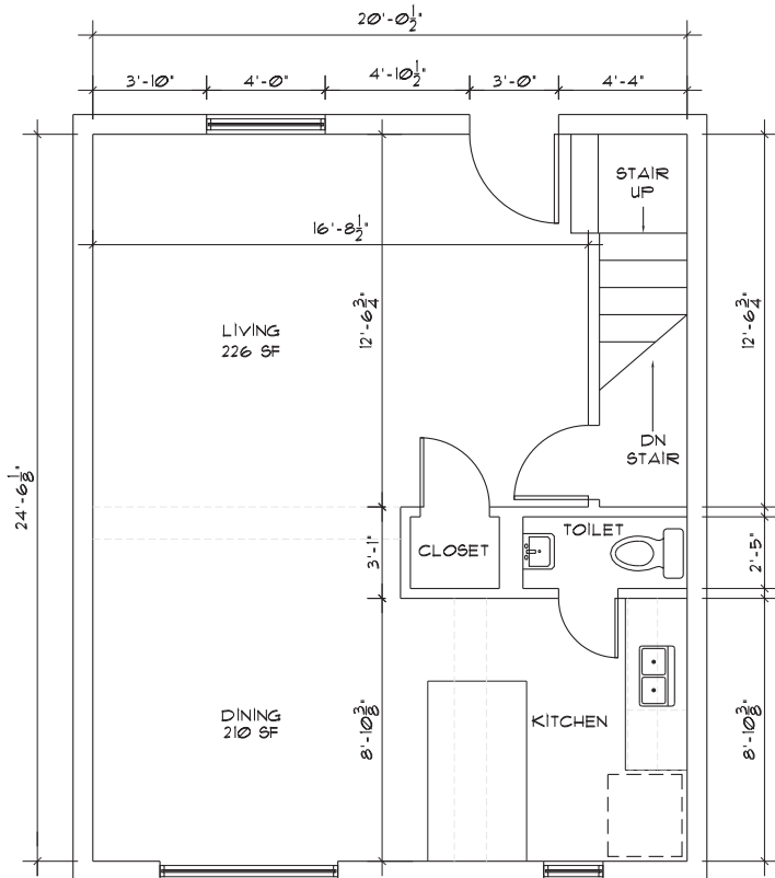
1st Floor Layout
