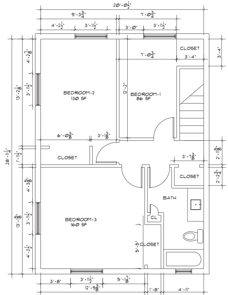
2nd Floor Layout
